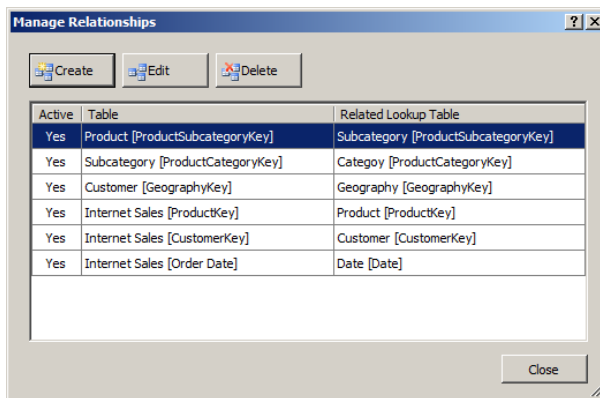
FIGURE 9-5 Manage Relationships dialog box displaying all relationships in the model
